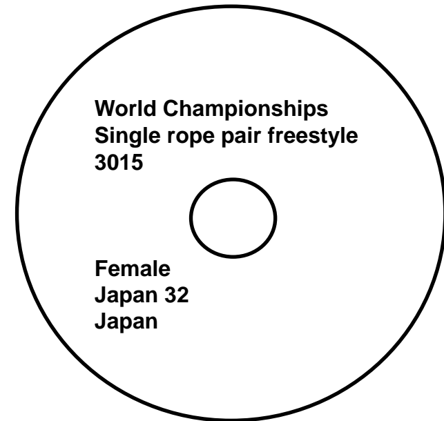
Teams example
